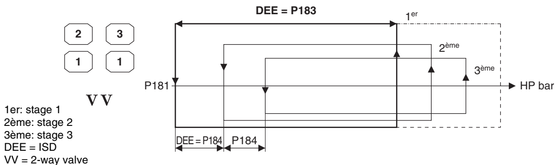
2 condenser fan modules per circuit = 3 single phase stages
