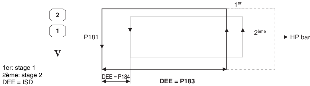
1 condenser fan module per circuit = 2 single-phase stages
