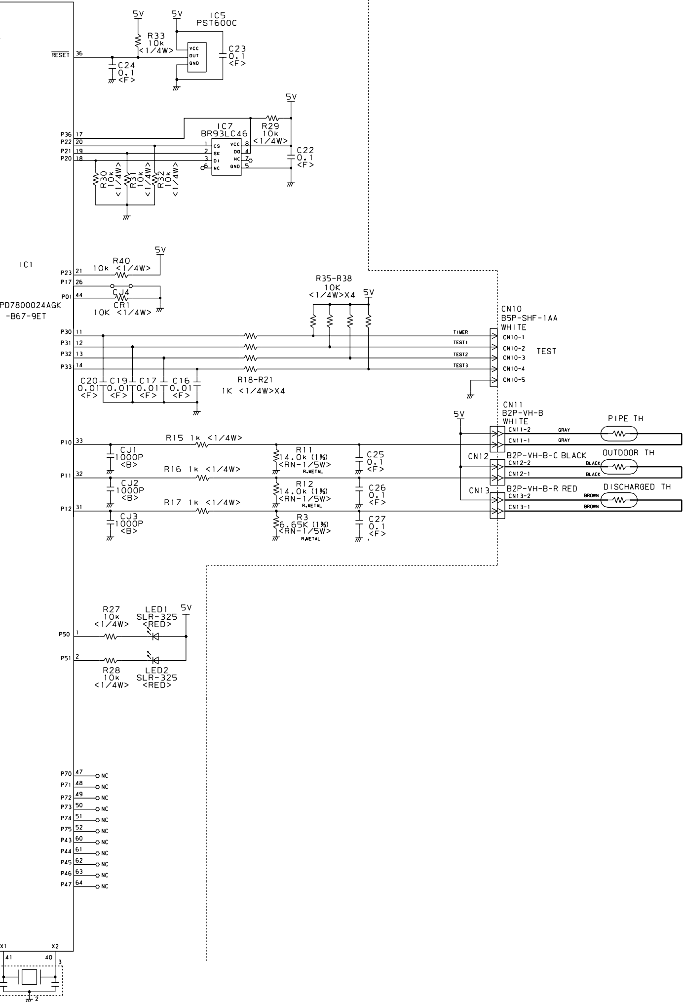
CONTROLLER PCB ASSEMBLY ( MAIN PCB ) EZ-0028HUE-C
