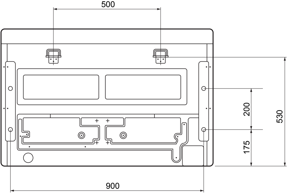
Rear view
