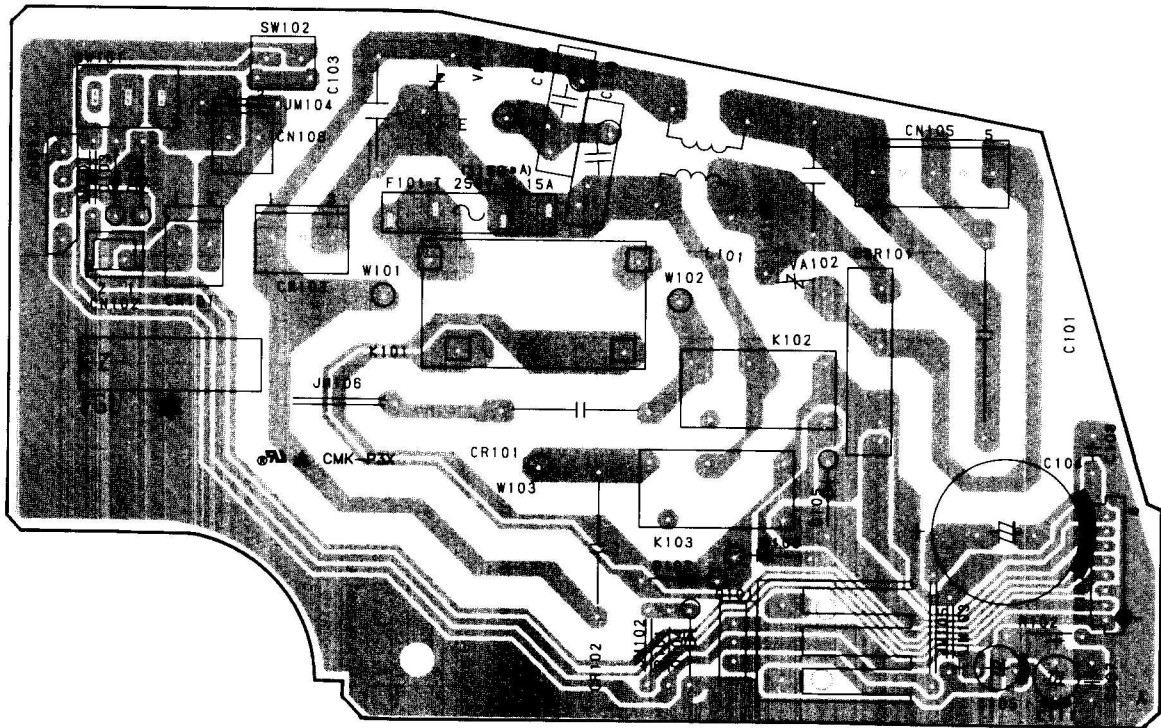
POWER SUPPLY PCB ASSEMBLY (VIEWED FROM THE SOLDER SIDE)
