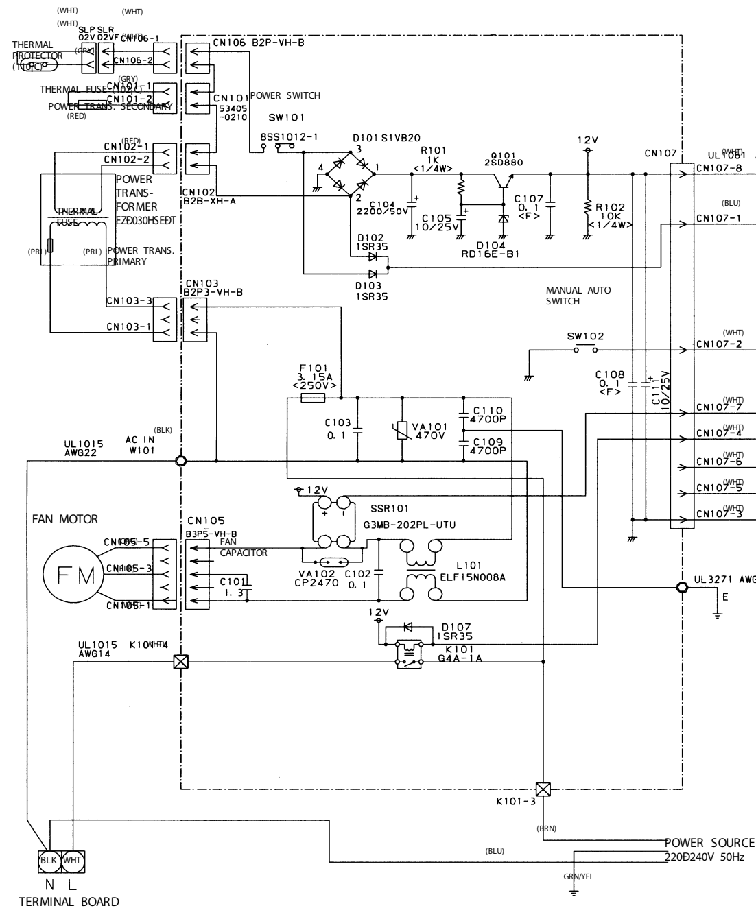
POWER SUPPLY PCB EZ-097VWSE-P
