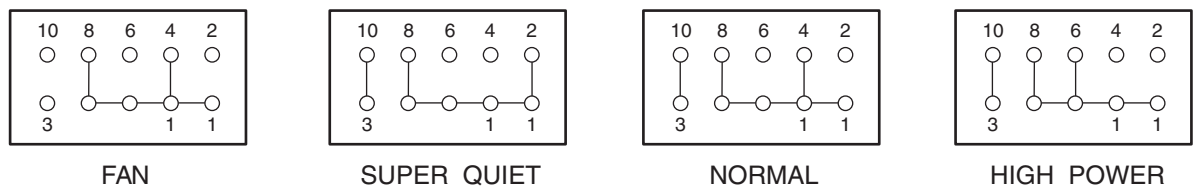
OPERATION SWITCH INTERNAL CONNECTIONS
