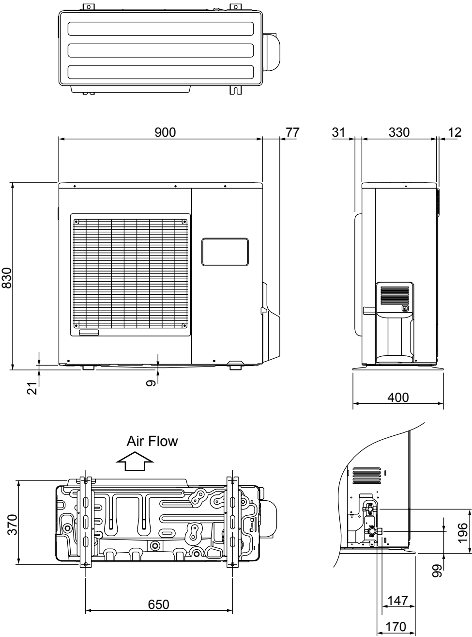
OUTDOOR UNIT
