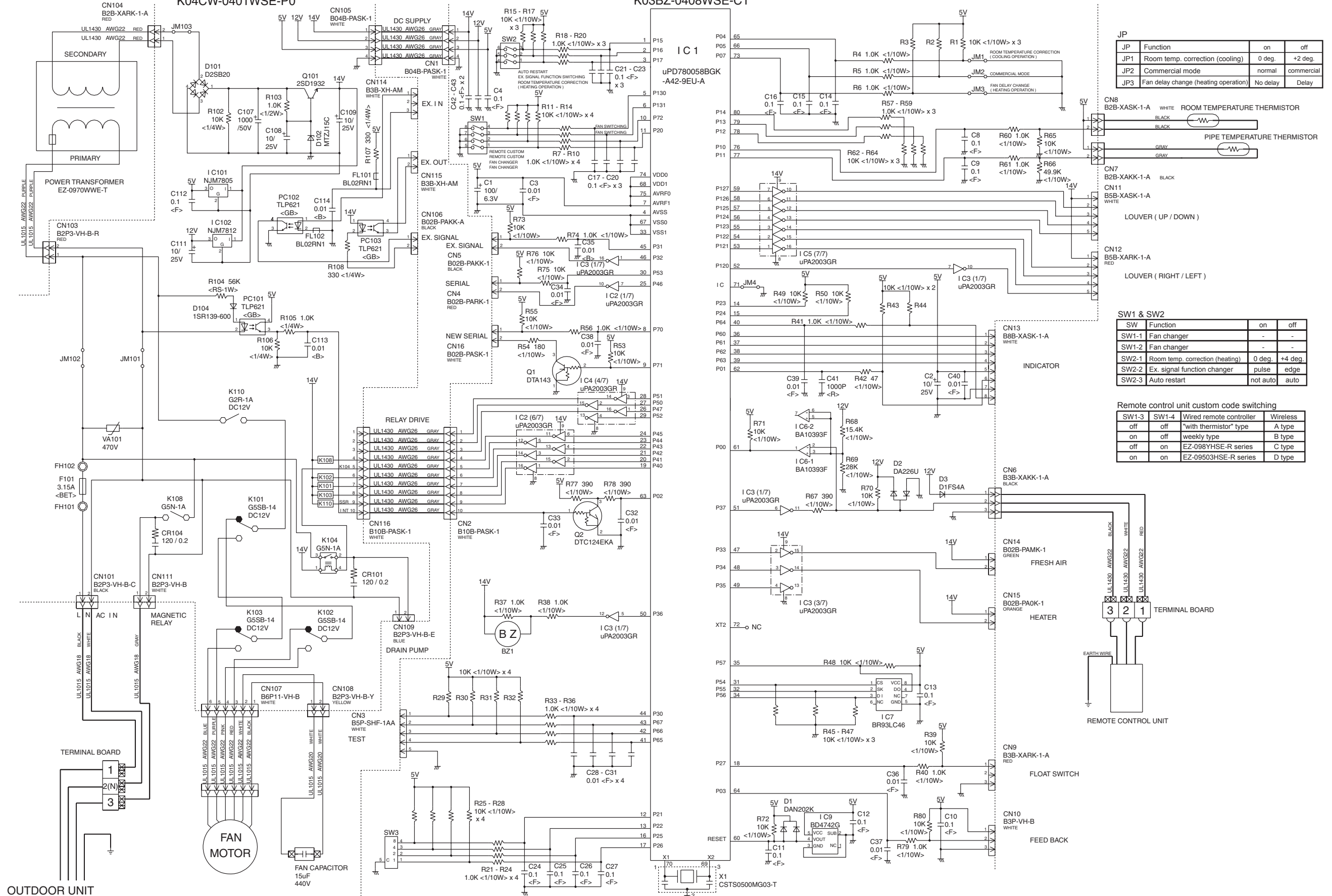
POWER SUPPLY PCB K04CW-0401WSE-PO
